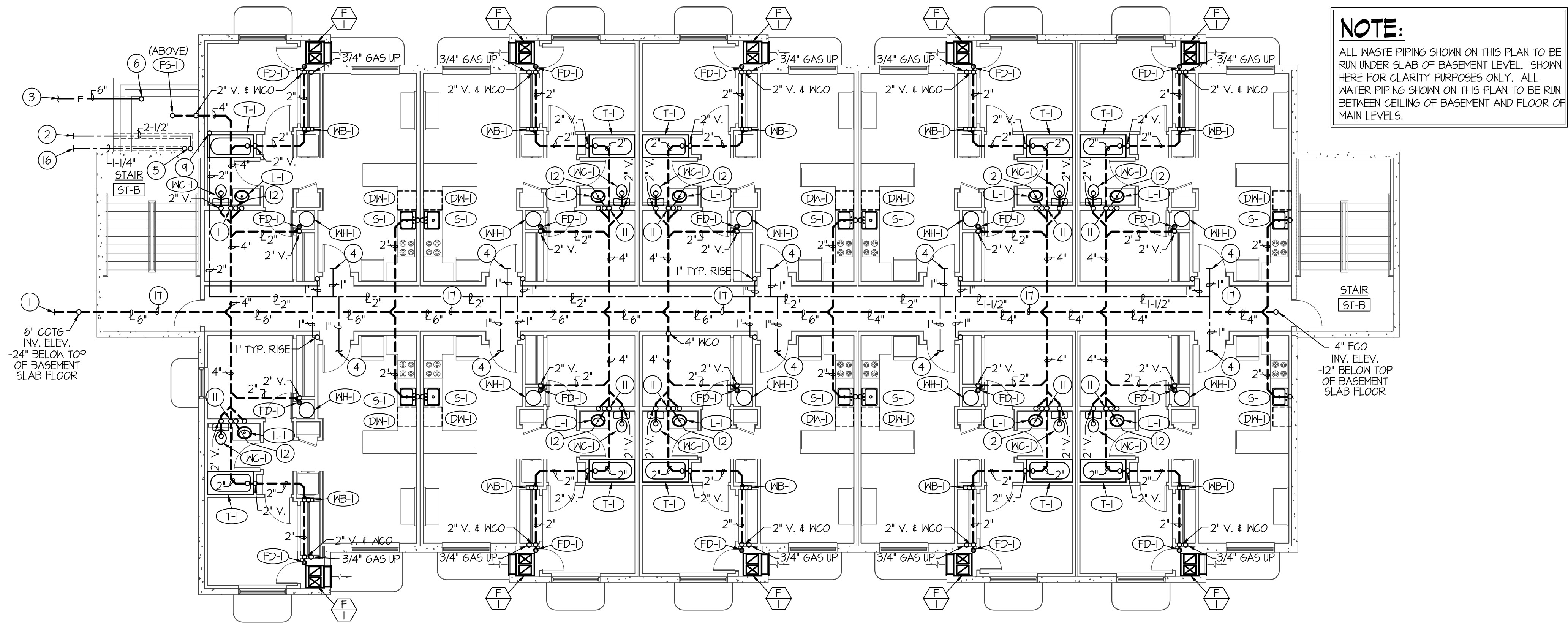
BLDG. I BASEMENT PLUMBING FLOOR PLAN
