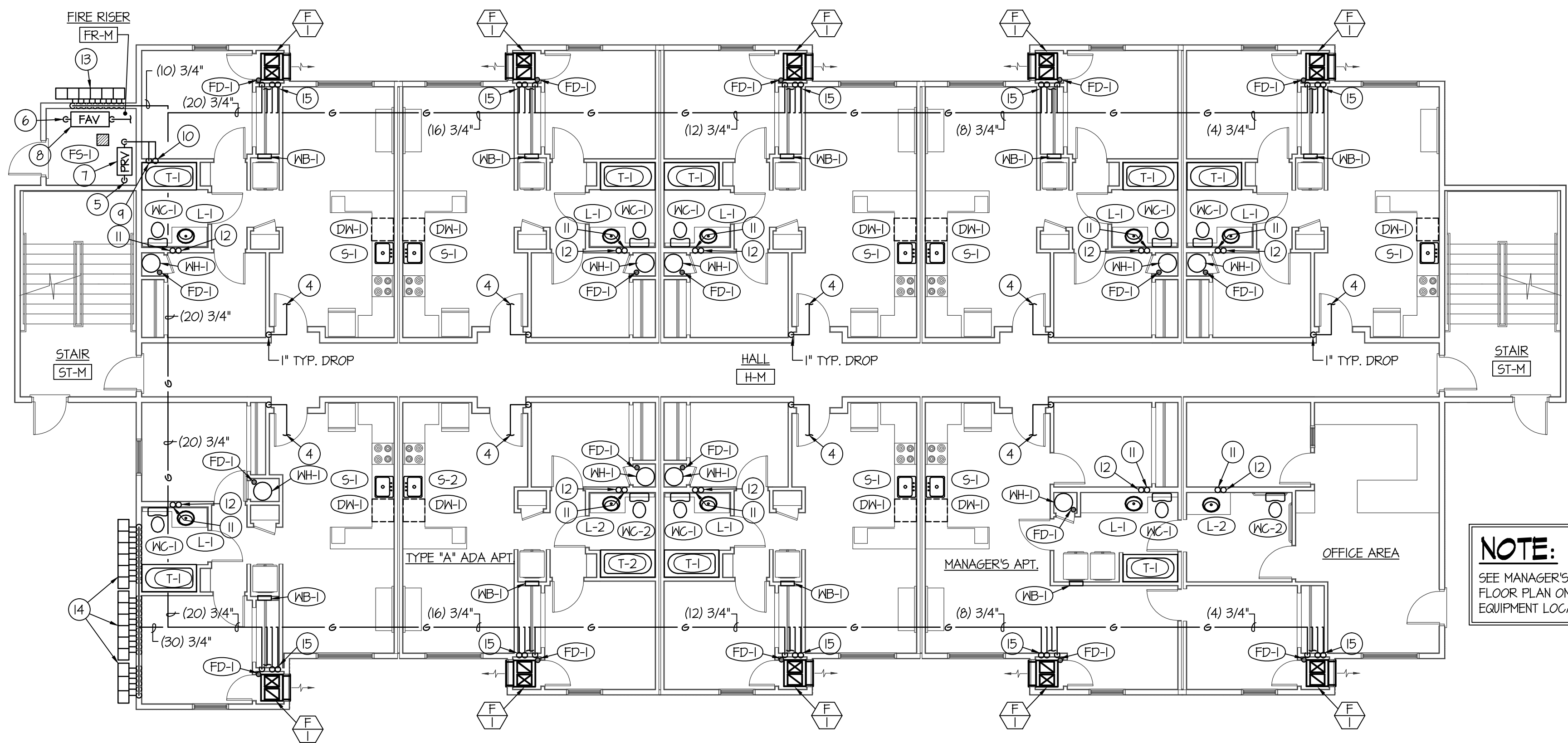
BLDG. I MAIN FLOOR PLUMBING PLAN
